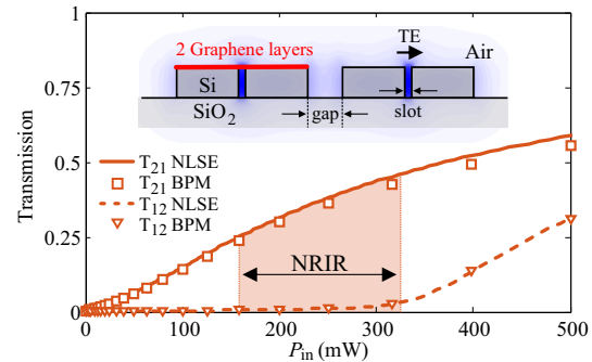
Figure 2. Forward (solid) and backward (dashed) transmission for the graphene waveguide coupler with SA. Shaded region corresponds to T_{21} \geq -6 dB and T_{12} \leq -15 dB. (Inset) Cross section (not to scale) of the silicon slot coupler with the symmetric supermode. The arrow indicates the dominant mode polarization.
