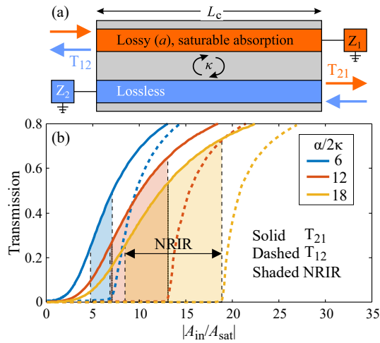
Figure 1. (a) Abstract two-port nonlinear asymmetric waveguide coupler of length L = L_c = \pi/2\kappa ; terminals Z_{1,2} denote matched loads. (b) Forward ( T_{21} ) and backward ( T_{12} ) transmission vs. normalized input amplitude; colors correspond to different values of the loss parameter \alpha/2\kappa .
