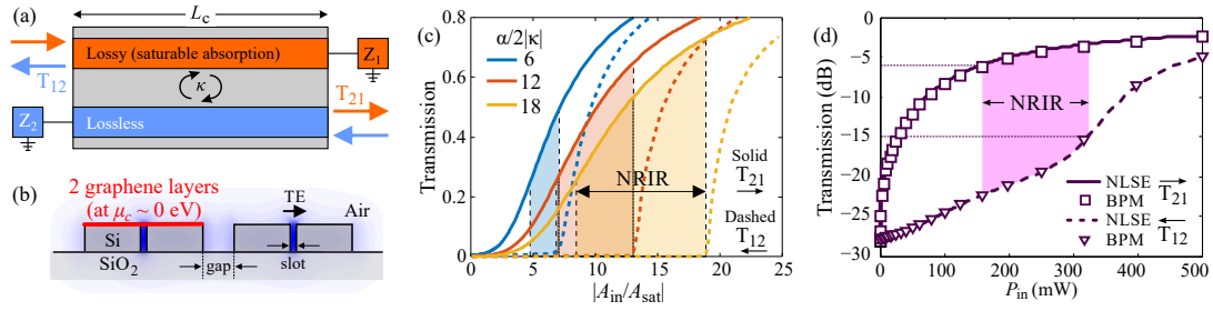
Fig. 1. (a) Abstract two-port nonlinear asymmetric waveguide coupler of length L = L_c = \pi/2|\kappa| ; terminals Z_{1,2} denote matched loads. (b) Proposed physical cross section (not to scale) of the silicon slot coupler with the symmetric supermode; the arrow indicates the dominant mode polarization. (c) Forward ( T_{21} ) and backward ( T_{12} ) transmission vs. normalized input amplitude using CMT; colors correspond to different values of the loss parameter \alpha/2|\kappa| . (d) Forward (solid) and backward (dashed) transmission for the graphene waveguide coupler with SA shown in (b), using coupled NLSE and BPM.
