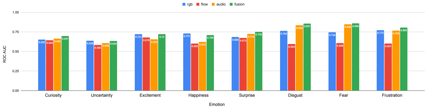
Fig. 2. ROC AUC per emotion, for each different modality and their average score fusion.
