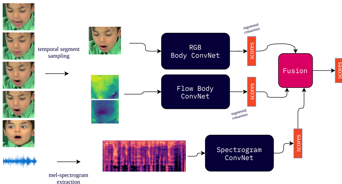
Fig. 1. The proposed multimodal emotion recognition architecture for child-robot interaction.
