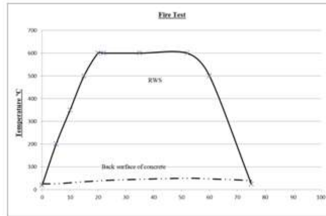
Figure 2: Temperature profile for fire test
