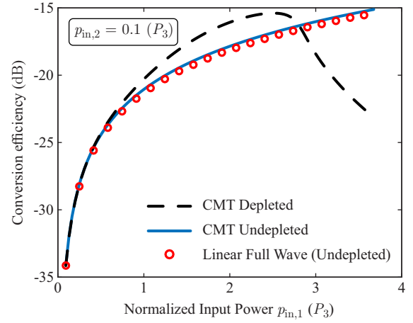
FIG. 3. Conversion efficiency of the DFWM process for the depleted (black dashed curve) and the undepleted pump case (CMT: blue solid curve, FEM: red markers). Depleted and undepleted pump calculations agree well for input powers as high as p_{\text{in},1} = 1 . CMT and full-wave calculations for the undepleted pump case are in excellent agreement, validating the developed framework. Self and cross nonlinear resonance frequency shifts have been neglected ( \gamma_{kl} = 0 in the CMT context).
