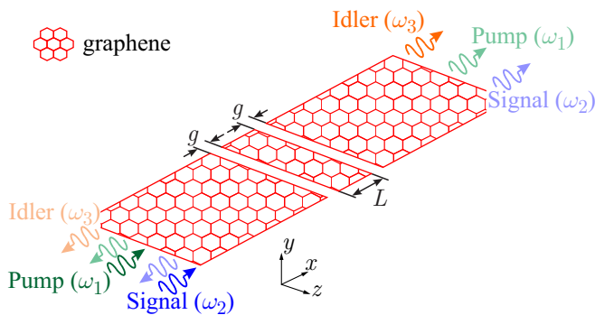
FIG. 1. Graphene plasmon-polariton standing-wave resonator of length L , directly-coupled with two semi-infinite graphene sheets, serving as the input/output waveguides through coupling gaps of length g . The nonlinear mixing of signal and pump waves generates a third wave (idler) through the DFWM process. Pale-colored waves carry comparable power with bright-colored waves but they are not presented in any illustration of the article. In addition, the pale-colored backward propagating idler wave at \omega_3 is not accounted for when calculating the conversion efficiency [Eq. (21)].
