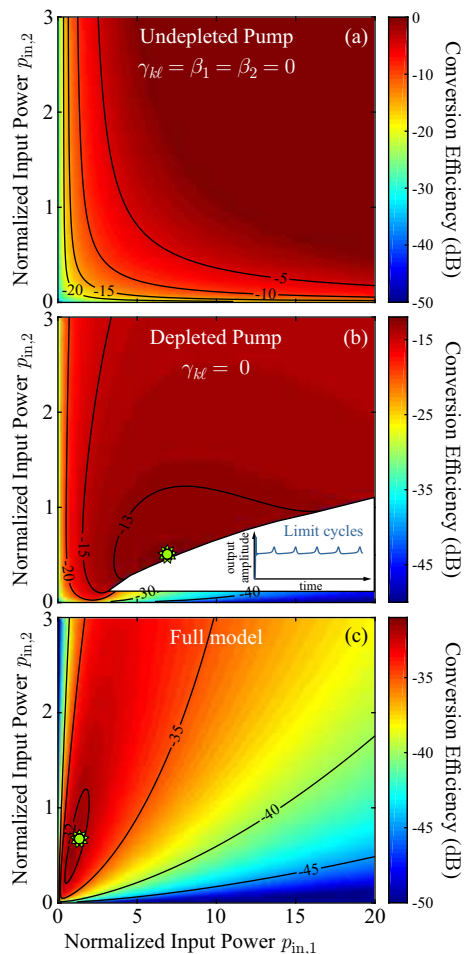
FIG. 4. Conversion efficiency of the DFWM process in the p_{\text{in},1} - p_{\text{in},2} space. (a) Undepleted pump case, (b) depleted pump case, and (c) full model including the nonlinear resonance frequency shifts due to SPM and XPM. In (b) maximum CE (star marker) equals -12.5 dB for p_{\text{in},1} = 7.0 and p_{\text{in},2} = 0.5 . In (c) maximum CE (star marker) equals -31.5 dB for p_{\text{in},1} = 1.0 and p_{\text{in},2} = 0.6 .
