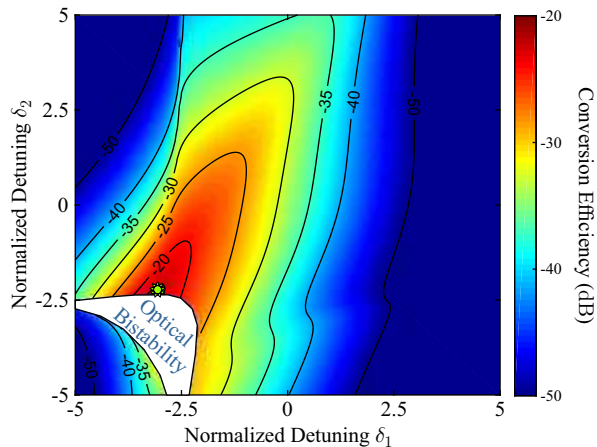
FIG. 5. Conversion efficiency of the DFWM process in the \delta_1 - \delta_2 space when all effects are taken into account. The power levels of the input waves are p_{\text{in},1} = 1.0 and p_{\text{in},2} = 0.6 . A maximum CE of -17.6 dB is obtained for \delta_1 = -3.10 and \delta_2 = -2.35 .
