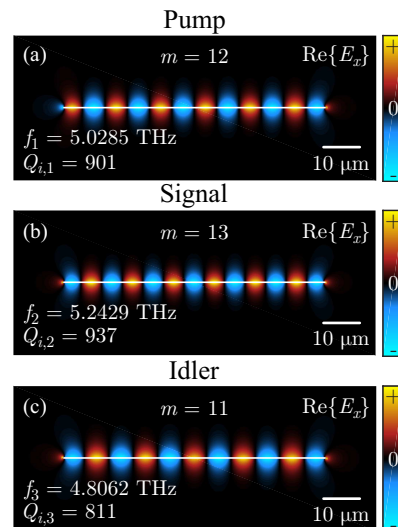
FIG. 2. Field plot ( E_x -component) of the resonance mode profiles supported by the graphene plasmon-polariton resonator. (a) m = 12 (pump wave), (b) m = 13 (signal wave), and (c) m = 11 (idler wave). It is noted that the three resonance frequencies are not exactly frequency-matched ( \omega_3 \neq 2\omega_1 - \omega_2 ) due to material dispersion.
