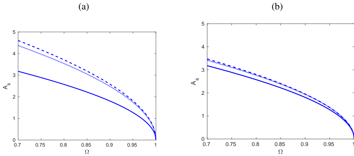
Figure 3. Graphs of the approximate critical amplitude at which supratransmission is triggered versus \Omega , for (a) \alpha = 2 and (b) \alpha = 3 . The parameters are as in previous figures. The solid curve is the short range interaction function (2.7), the dashed lines are the numerical approximations, and the dotted curve is the plot of the empirical formula (4.2).
