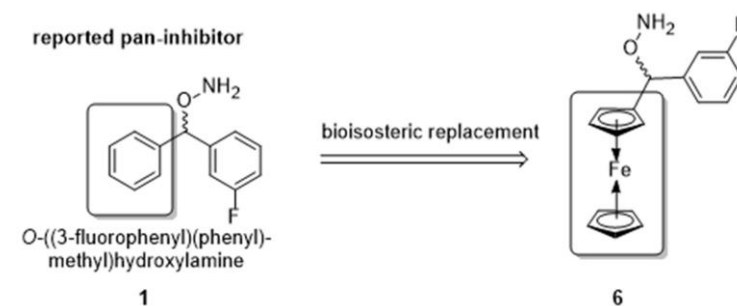
Figure 1. Bioisosteric replacement of a phenyl group with ferrocenyl moiety on a known KP pan-inhibitor.
