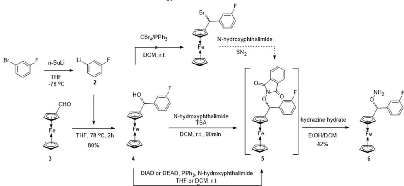
Scheme 1. Synthesis of the ferrocenyl analogue 6 .
