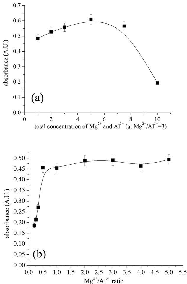
Fig. 2 Effect of the Mg^{2+}/Al^{3+} concentration (a) and ratio (b) on extraction. Conditions: 15.8 nmol\ L^{-1} of citrate-capped AuNPs (4 nm), 100 mmol\ L^{-1} KOH, room temperature, 1 min mixing time, centrifugation for 30 min at 6000 rpm (4200 g), dissolution in 0.5 mL of 0.5 mol\ L^{-1} HCl.
